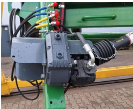
Autonomous oil station on ZRM-180. To increase the flow of oil on the hydraulic motor.
